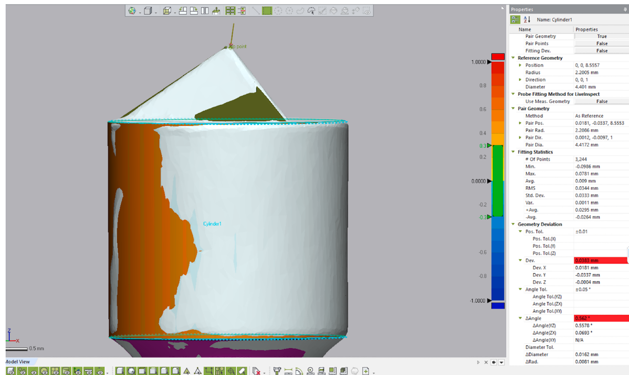
Fig. 5. CMM point marked on top of the pyramid on the SB to measure linear deviations and cylinder (dashed turquoise line) generated to measure angular deviations.
