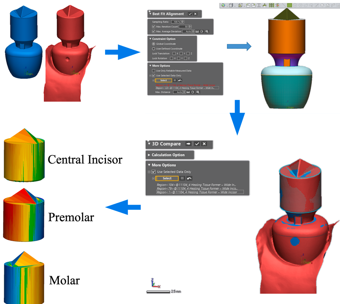
Fig. 4. Overview of superimposition process. Blue CHA-SB represents library CAD file (CHA-SB-LIB-STL) and red CHA-SB represents test scan file (CHA-SB-T-STL).
