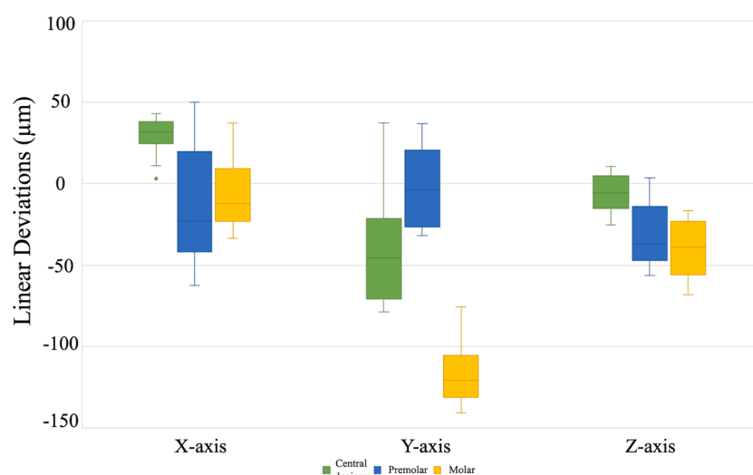
Fig. 6. Box-plot graph of raw linear deviations of each implant location-axis pair.
