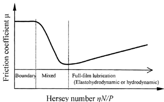
FIGURE 6 Stribeck curve, showing the friction coefficient against the Hersey number with three different regimes, boundary, mixed and full-film lubrication (Woydt & Wäsche, 2010). Horizontal axis is the \eta N/P , where \eta stands for viscosity, N relative speed of the surfaces and P as the load on the interface per unit
