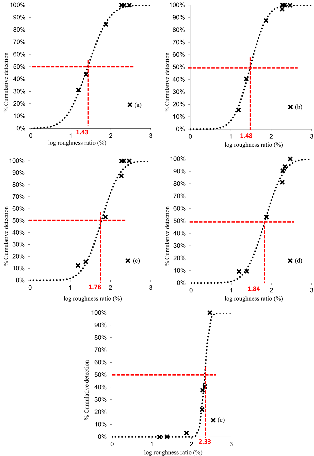
FIGURE 2 Log-normal fitting (probit analysis) of the cumulative population percentage vs the roughness ratio at room temperature (25C) for: (a) in air (Median: 10^{1.43} = 29\% ), (b) in water (Median: 10^{1.48} = 30\% ), (c) in 80% syrup (Median: 10^{1.78} = 60\% ), (d) in 90% syrup (Median: 10^{1.84} = 63\% ), and (e) in 100% syrup (Median: 10^{2.33} = 216\% )
