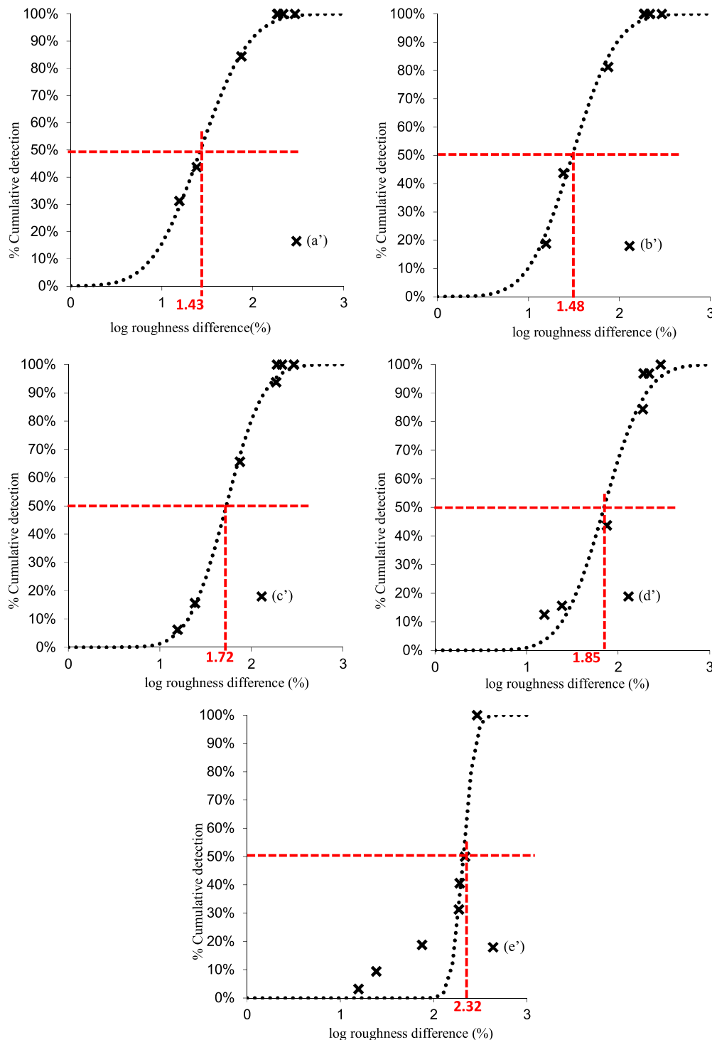
FIGURE 4 Log-normal fitting (probit analysis) of the cumulative population percentage vs the roughness ratio at 37C for B', C', D' and E' and 25C for A, for (a) in air (Median: 10^{1.43} = 29\% ), (b') in water (Median: 10^{1.48} = 30\% ), (c') in 80% syrup (Median: 10^{1.72} = 53\% ), (d') in 90% syrup (Median: 10^{1.85} = 70\% ), and (e') in 100% syrup (Median: 10^{2.32} = 207\% )
