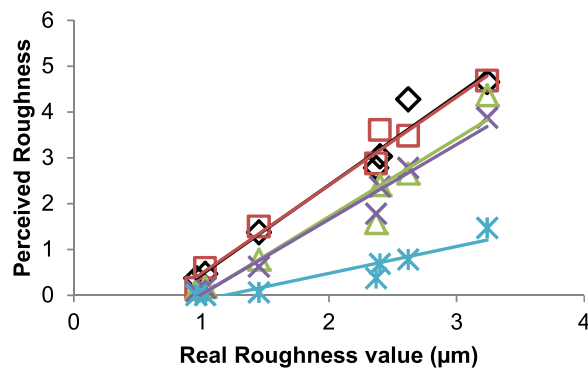
FIGURE 7 Average scores of the roughness values against the real roughness value for the different conditions of air, water, 80, 90, and 100% syrup, at 25C
