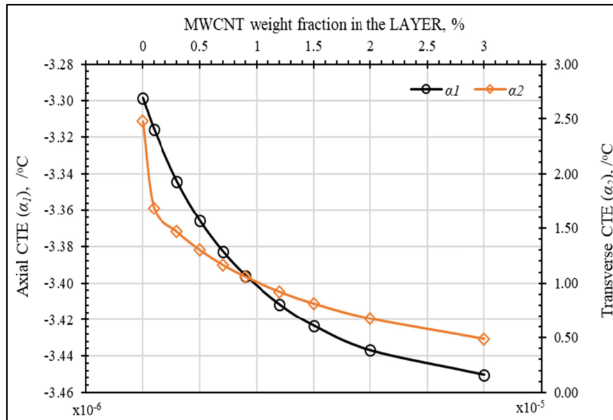
Figure 4. Change of the longitudinal and transverse thermal expansion coefficients of the layers according to MWCNT ratio
