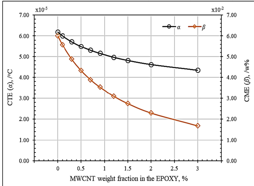
Figure 3. Change of the hygrothermal coefficients of the epoxy according to MWCNT ratio
