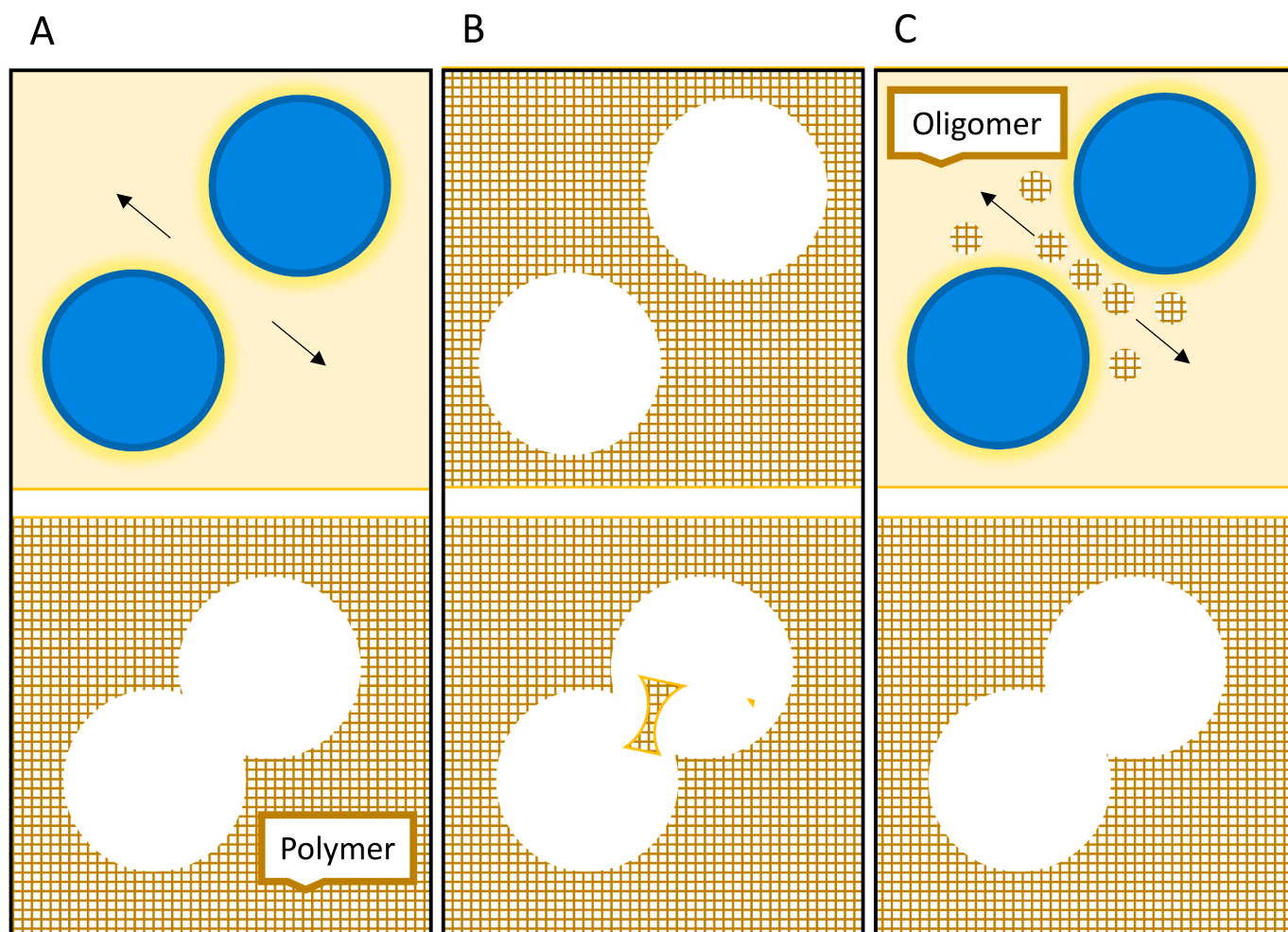
Fig. 12. The three proposed pore throat formation mechanisms in conventional polyHIPEs: (A) The drainage or rupture of the thin interfacial continuous film during polymerization (arrows indicates drainage from interface to Plateau border), (B) the thin polymer film between the pores of the polyHIPE is being ruptured during the post processing of the material, (C) the growing oligomer chains at the interfacial area migrate to the Plateau border where this migration induces depletion forces so that the emulsion droplets semi-coalesce during the polymerization (arrows indicate the migration of the oligomers).
