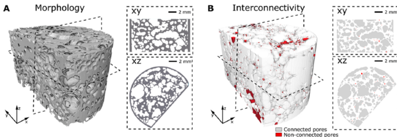
Fig. 20. The reconstructed 3D image and the 2D images from two different planes of a polyHIPE obtained from \mu CT (reproduced from [137]).
