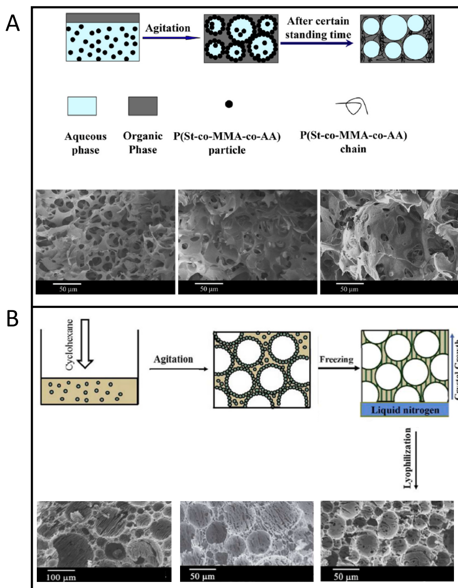
Fig. 18. (A) The schematic representation of the formation of anti-Finkle emulsion where the stabilizing particles are dispersed in the internal phase initially. As the particles interact with the continuous phase where they are soluble, particles disintegrate into polymeric chain and forming the material skeleton. The SEM images of the anti-Finkle emulsion templates demonstrating the loss of interconnectivity of the HIPE template as the standing time of the HIPE increase; 0, 24 and 48 h after preparation from left to right (reproduced from [125]). (B) A schematic representation of the channel formation in Pickering emulsion template by unidirectional freezing. The SEM images of the obtained templates and the effect of the increasing particles concentration (15, 25 and 30 %wt particle concentration from left to right) on the channel formation. Adapted with permission from [127]. Copyright 2016 American Chemical Society.
