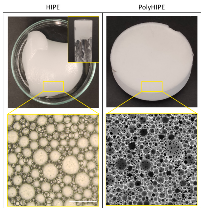
Fig. 7. The digital images of highly viscous, self-supporting HIPE and its optical micrographs (left). The photopolymerized 3D polyHIPE and its SEM image of the internal structure. Scale bars are 200 \mu\text{m} .
