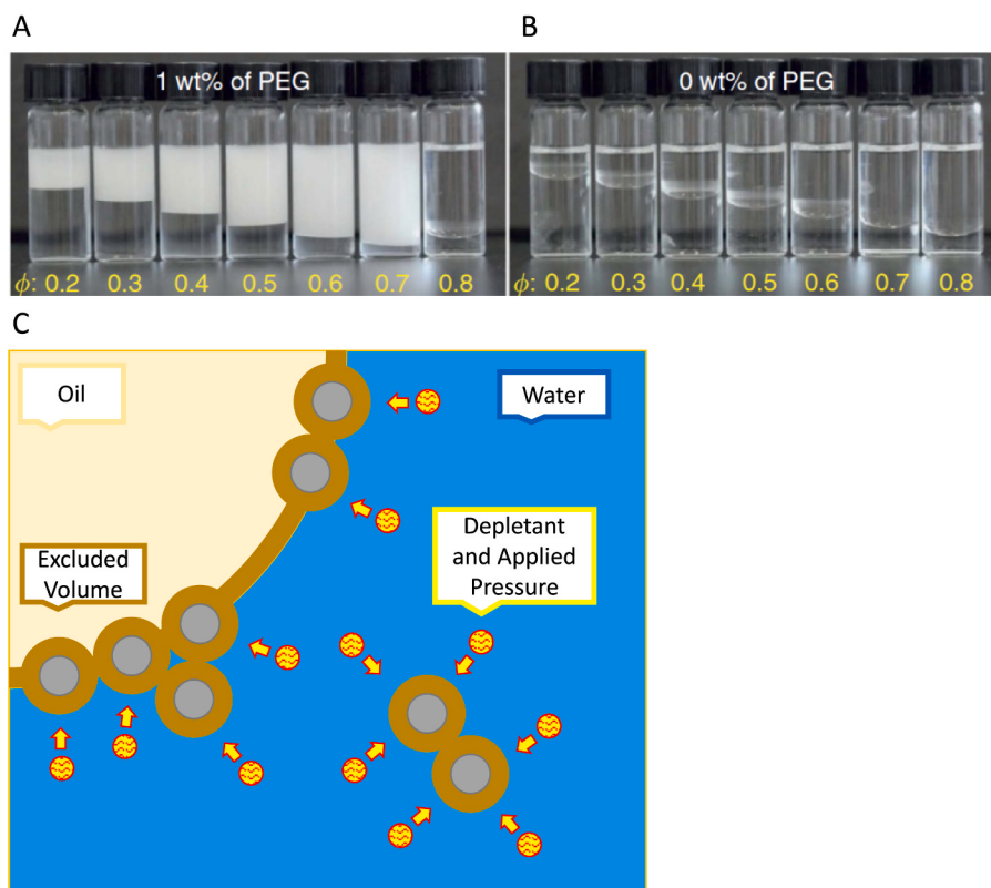
Fig. 3. The preparation of emulsion by exploiting depletion attraction: (A) The digital images of formation of Pickering HIPE at various internal phase fraction in the presence of depletant PEG and (B) their phase separated counterparts in the absence of depletant agent. Adapted with permission from [19]. (C) The schematic representation of achieving stability with depletion attraction (redrawn from [19]).
