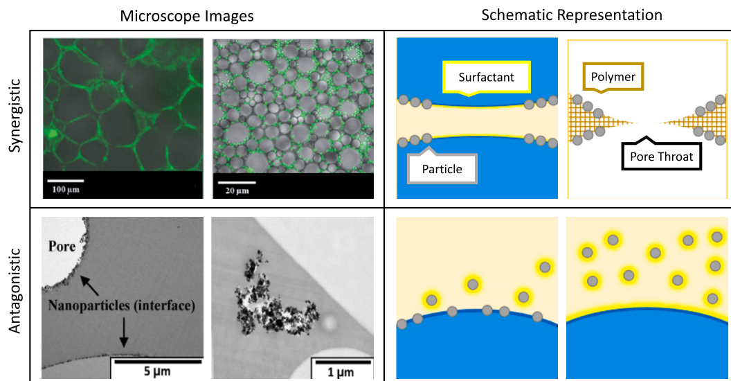
Fig. 14. Representation of proposed synergistic and antagonistic effect of dual emulsifier system. Synergistic effect demonstrated with confocal microscopy where the green fluorescent particles as a sole stabilizer covering the emulsion droplets (left), when the surfactant is used as co-emulsifier, particles are found at the highly curved regions of the emulsion droplets (right) (reproduced from [104] with permission from the Royal Society of Chemistry). The synergistic effect is schematically represented, where the surfactant molecules are located at the less curved region of droplets (left). These regions are susceptible to thin film rupture during polymerization, leading to the formation of pore throats (right). Alternatively, antagonistic effect of dual emulsifier system is represented in TEM images of polyHIPE. Particles as a sole HIPE stabilizer localize at the interface (left) however, when the surfactant is used, the particles are observed within the polymer in an aggregated form (right) (Adapted with permission from [113]. Copyright 2014 American Chemical Society). The antagonistic effect is schematically represented where the surfactant is adsorbed on the particle surface first and de-attaches them from the interface (left) and surfactant function as a stabilizer only when the particle surfaces are saturated with surfactant (right). (For interpretation of the references to colour in this figure legend, the reader is referred to the web version of this article.)
