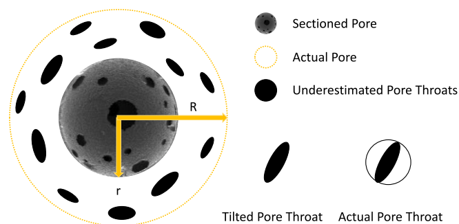
Fig. 19. Schematic representation of uneven sectioning of polyHIPEs. R and r represents the actual and the sectioned radius of the pores.
