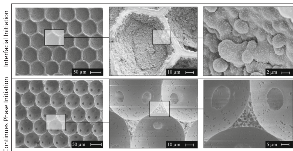
Fig. 9. The changes in conventional polyHIPE morphology caused by the difference in locus of initiation; closed polyhedral pores with rough pore surface are obtained in interfacial initiation, while spherical interconnected pores with a smooth pore surface are obtained in continuous phase initiation. Adapted with permission from [89]. Copyright 2017 American Chemical Society.
