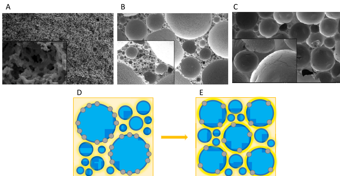
Fig. 15. SEM images of polyHIPEs: (A) PolyHIPEs obtained from HIPE stabilized by surfactant, (B) dual emulsifier and (C) colloidal particles. (B) The hierarchical porous structure is obtained when both surfactant and colloidal particles are used to stabilize HIPE (reproduced from [99]). Schematic representation of interplay between surfactant and colloidal particle concentration on the HIPE/polyHIPE morphology: (D) When the particle/surfactant ratio is high, large pores are mainly stabilized by colloidal particles, (E) when the particle/surfactant ratio is low, average droplet/pore size reduces.
