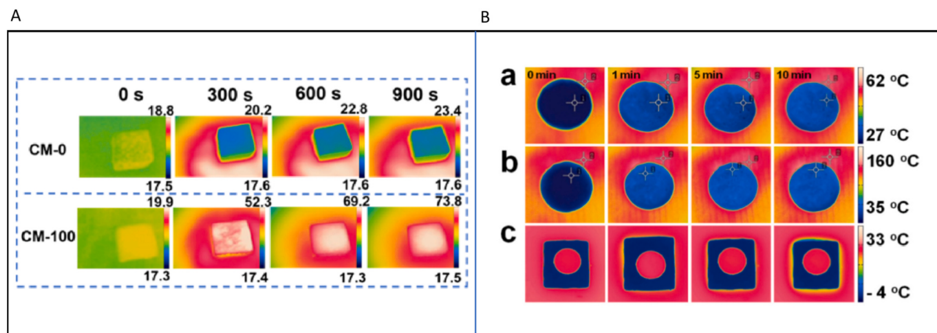
Fig. 21. (A) The infrared images of polyHIPE (CM-0) and carboxylated CNT incorporated Pickering polyHIPE (CM-100) captured at different times under light irradiation, demonstrating to light-to-heat conversion of CNT incorporated Pickering polyHIPE. Adapted with permission from [168]. Copyright 2022 American Chemical Society. (B) The infrared images of polyHIPE demonstrating their low thermal conductivity: PolyHIPE on a hot plate (a), and on ice (c) (reproduced from [171]).
