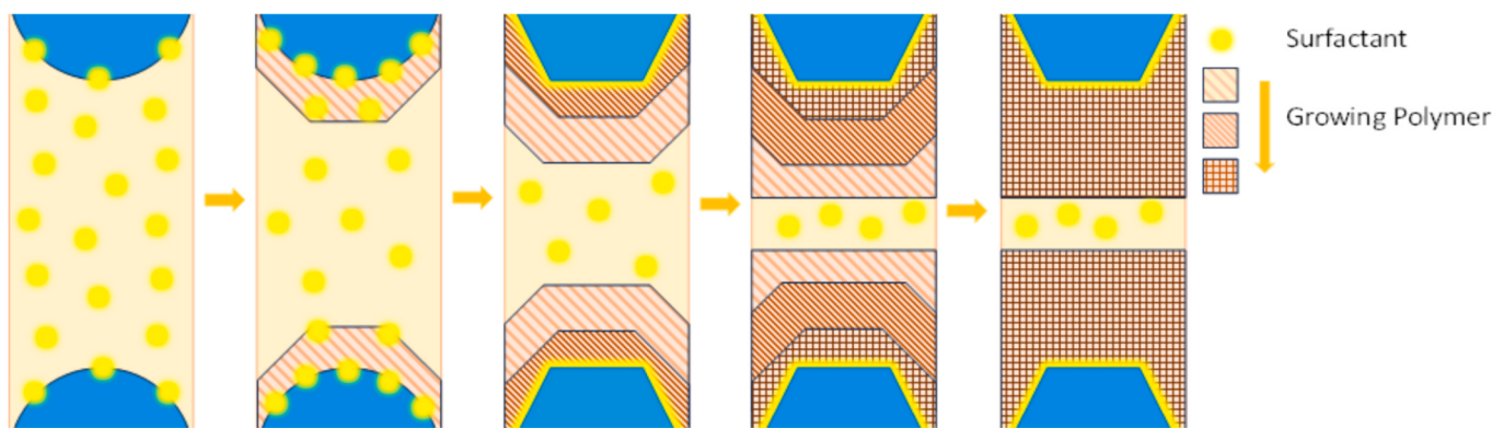
Fig. 10. Schematic representation of pore shape changes from spherical to hexagonal in during the interfacial polymerization of HIPE. The figure is redrawn from [92].
