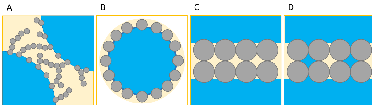
Fig. 6. The schematic representation of mechanisms involved in increased Pickering HIPE elastic modulus: (A) Interparticle interaction forming 3D network in interfacial area, (B) excluded volume effect, (C, D) lateral capillary interactions between particles. Figures are redrawn from [52].
