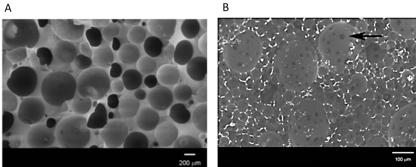
Fig. 17. (A) Closed cellular PolyMIPE when the CNT is the sole emulsion stabilizer, (B) open cellular PolyMIPE obtained by HIPE stabilized by CNT dispersed in the oil phase and the oxidized CNT dispersed in the water phase (black arrow indicates the pore throat). Adapted with permission from [118]. Copyright 2007 American Chemical Society.
