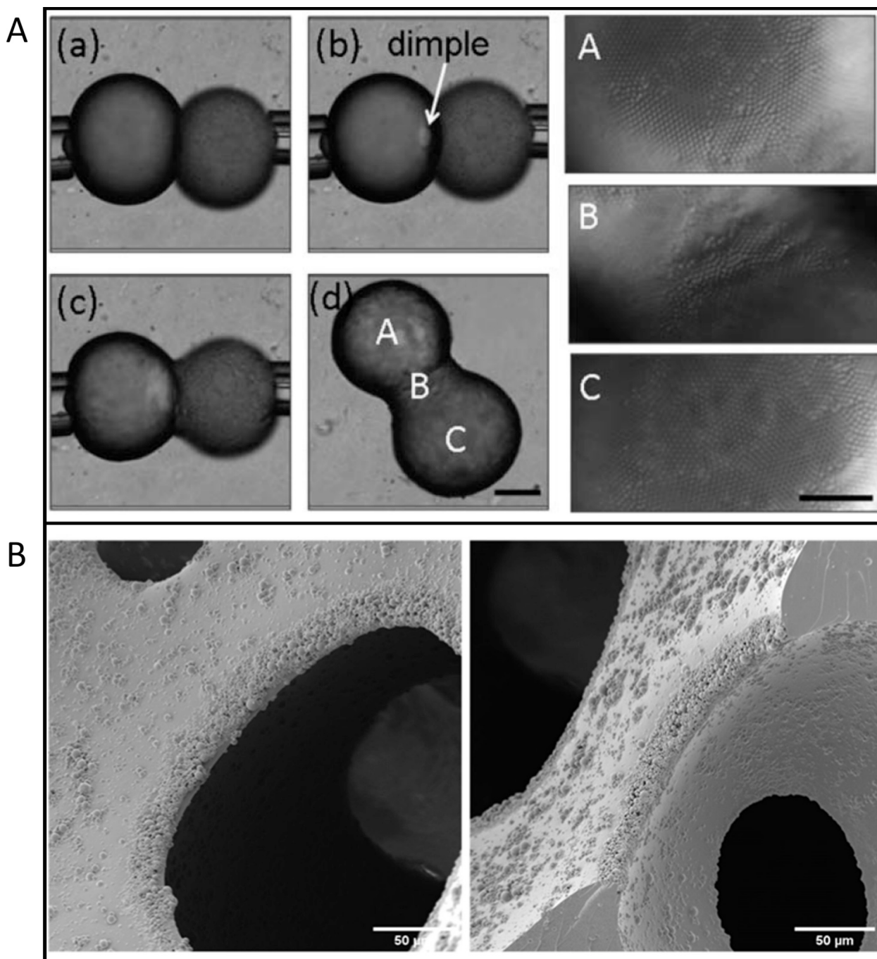
Fig. 13. (A) Manipulation of sparsely covered hexadecane emulsion droplets via micropipette to contact with each other and the formation of dimple at the contact region between two droplets [17]. (B) Proposed pore throat formation in Pickering PolyHIPE via arrested coalescence where the pore throats are crowded with particles indicating the dimple formation prior to polymerization [97].
