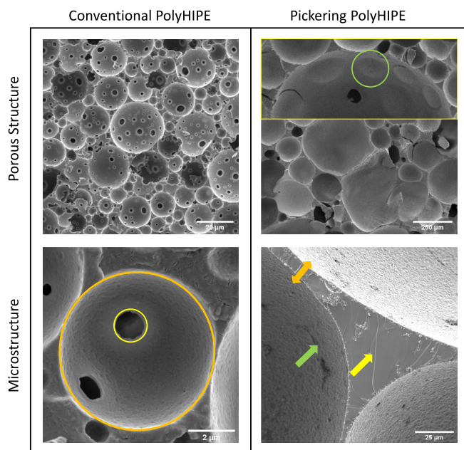
Fig. 8. SEM Images of typical polyHIPEs obtained by surfactant-stabilized (conventional polyHIPEs) or colloidal particle-stabilized HIPEs (Pickering polyHIPEs). Overall porous structure of a conventional polyHIPE; pores and pore throats are 10 and 1 \mu\text{m} , respectively. The orange circle highlights a pore, an imprint of HIPE droplets after being polymerized and internal phase removal. The yellow circle highlights a typical pore throat. Overall porous structure of a typical Pickering polyHIPE with \sim 100 \mu\text{m} pores without interconnecting pore throats. The green circle highlights the thin polymeric film covered pore throats. The orange arrows show the interfacial polymeric film separating two neighboring pores, the green arrow shows the pore surface and the yellow arrow shows the polymerized trigonal region (Plateau border), the intersect of three pores. (For interpretation of the references to colour in this figure legend, the reader is referred to the web version of this article.)
