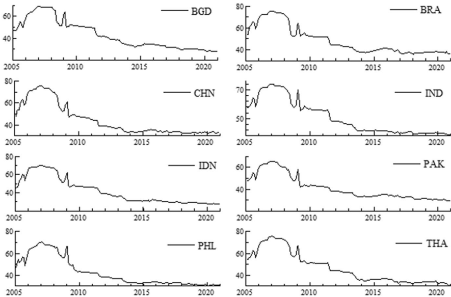
Fig. 2 Dynamic total connectedness index
