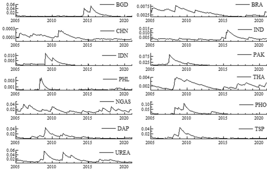
Fig. 1 The plots of EWMA-based volatility series
