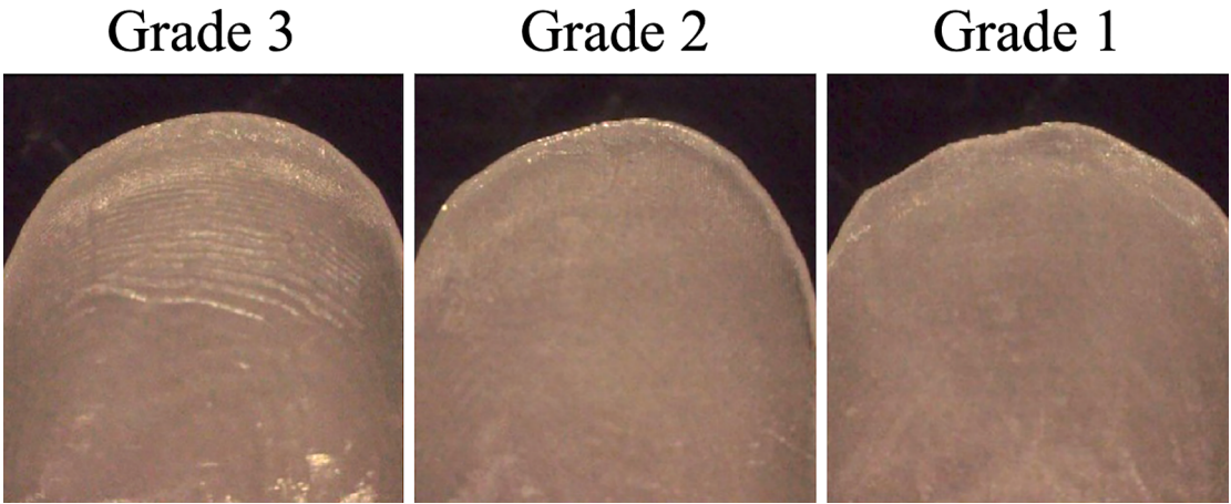
Fig. 4. Representative stereomicroscope images used to evaluate margin quality of tested laminate veneers. Three-point scale used ranged from 3 (high marginal quality) to 1 (low marginal quality) and images show labial margin quality.
