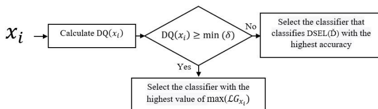
Figure 5. DCS-DQ method.
