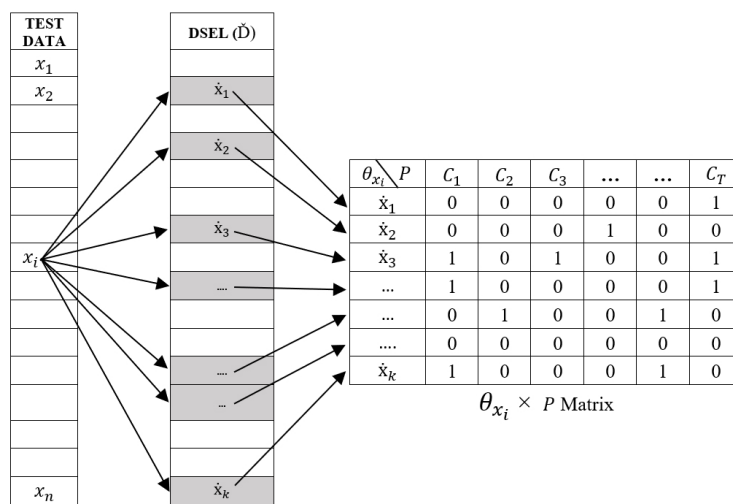
Figure 4. Proposed dynamic classifier selection method DCS-DQ.
