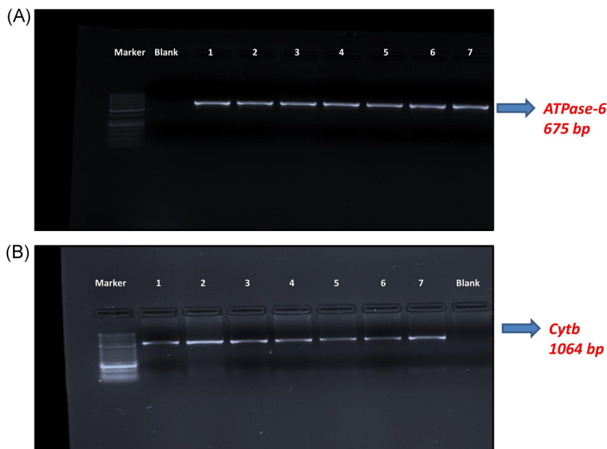
FIGURE 1 ATPase-6 and CYB gel electrophoresis image
